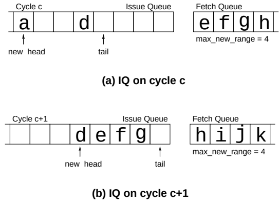
Figure 2. Operation of new_head pointer and max_new_range
