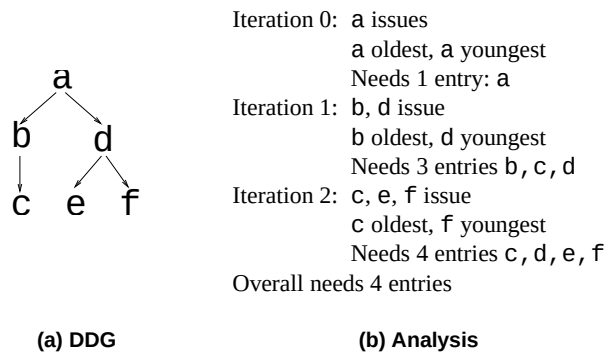
Figure 3. Determining the number of IQ entries needed in a DAG
