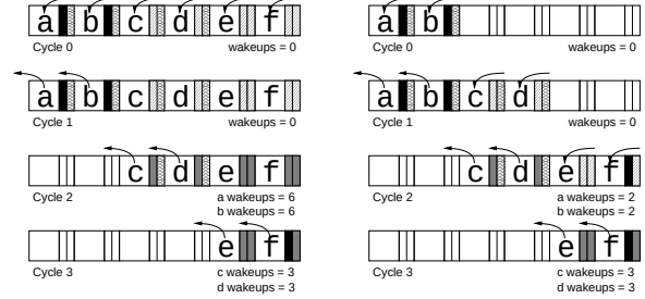
(c) The normal IQ
