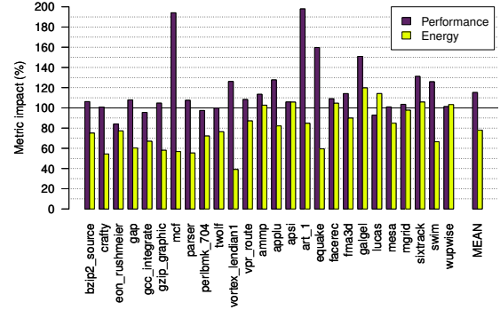
Figure 5. Performance and energy breakdown for our model when using the advanced features compared to the best overall static configuration. On average performance is improved by 15% and energy reduced by 21%.
