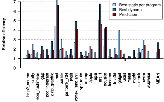
Figure 6. Energy-efficiency achieved by our model for all of SPEC CPU 2000 compared to the best static configuration tailored for each program and compared with the best dynamic configuration tailored for each program’s phase. All the values are normalised by the best overall static configuration (higher is better).
