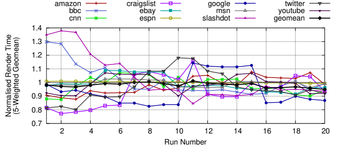
(b) The execution time of twenty rounds of BBench, normalised to overall average render time for each page. We see that there is no pattern – MarkUs does not cause increasing slowdowns over time.
