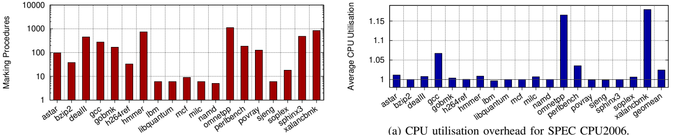
Fig. 7: Number of marking procedures performed in each SPEC CPU2006 workload.
