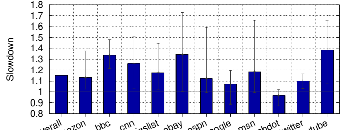
(a) Slowdown for BBench. Error bars show the range of load times from each successive page load, and result from marking procedure costs not being evenly shared across all pages, in addition to existing variance even without MarkUs.
