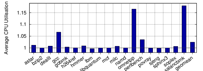
(a) CPU utilisation overhead for SPEC CPU2006.
