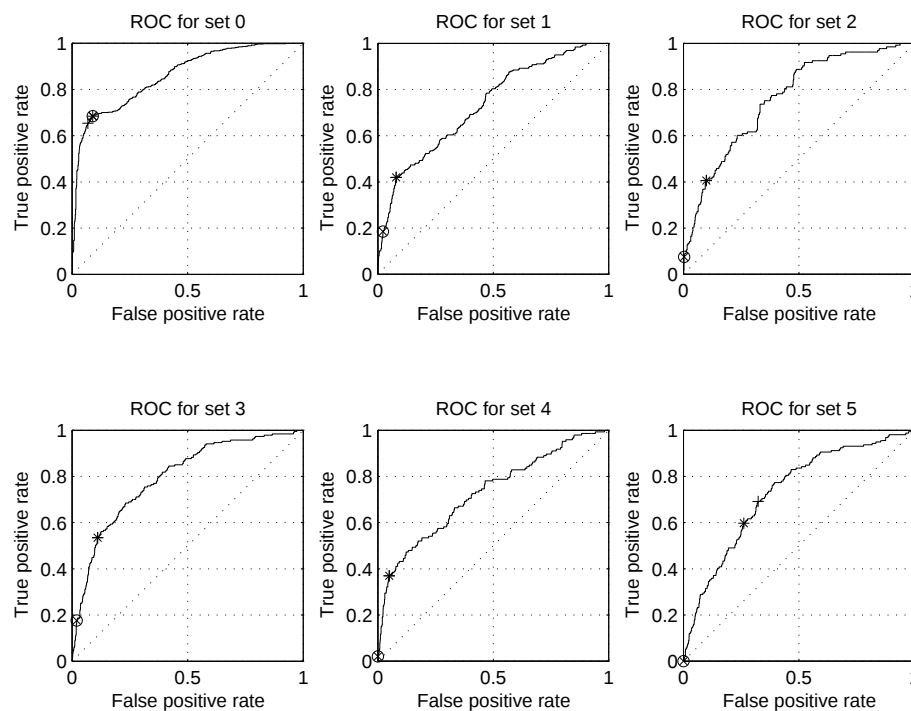
Fig. 6 ROC curves for the individual heuristic classifiers, evaluated using the validation sets, for classifiers trained using all features. In each case, a circle indicates the optimal ROC operating point, a cross the point corresponding to maximum accuracy, a star maximum F1, and a plus maximum Matthews
