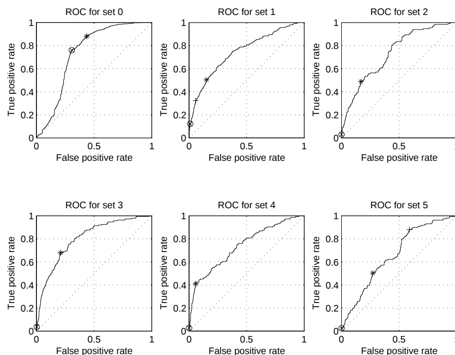
Fig. 8 ROC curves for the individual heuristic classifiers, evaluated using the validation sets, for classifiers trained using only dynamic features. In each case, a circle indicates the optimal ROC operating point, a cross the point corresponding to maximum accuracy, a star maximum F1, and a plus maximum Matthews
