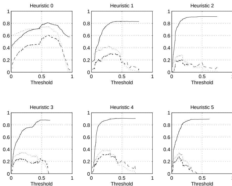
Fig. 4 Variation of performance measures with threshold t , evaluated using the validation sets, for classifiers trained using only static features. The solid line shows accuracy, the dotted line F1 and the dashed line Matthews
