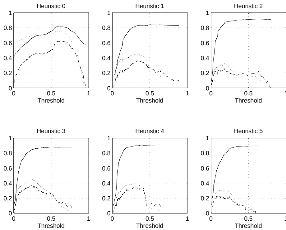
Fig. 3 Variation of performance measures with threshold t , evaluated using the validation sets, for classifiers trained using all features. The solid line shows accuracy, the dotted line F1 and the dashed line Matthews
