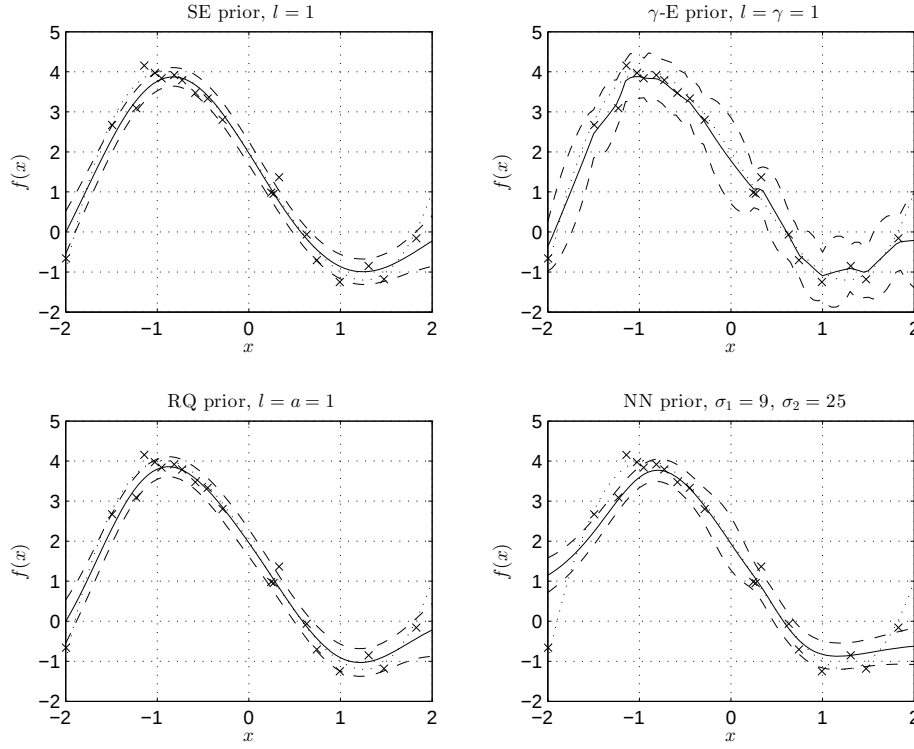
Fig. 2 The mean and variance of the predictive distribution for Gaussian process regression using the covariance functions in Table 10. The dotted line shows the polynomial p(x) and the crosses show the training examples. See the text for an explanation of the solid and dashed lines
