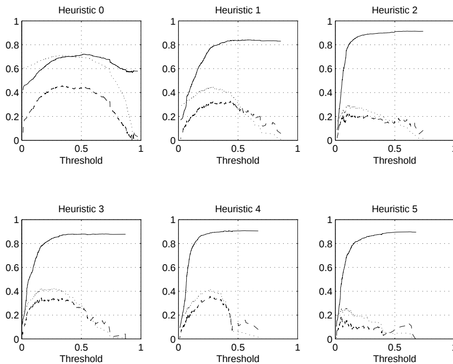
Fig. 5 Variation of performance measures with threshold t , evaluated using the validation sets, for classifiers trained using only dynamic features. The solid line shows accuracy, the dotted line F1 and the dashed line Matthews
