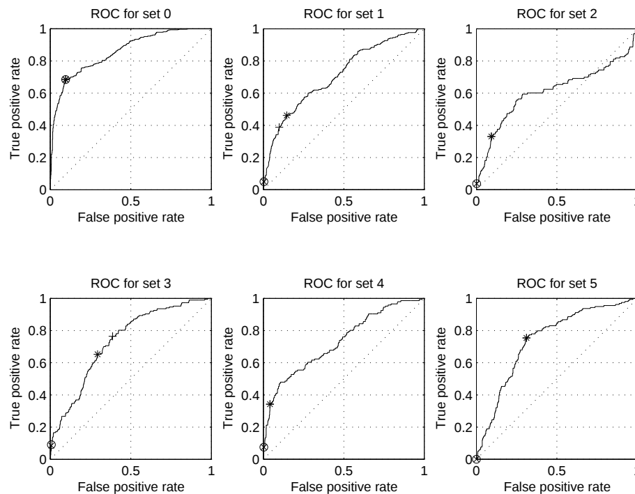
Fig. 7 ROC curves for the individual heuristic classifiers, evaluated using the validation sets, for classifiers trained using only static features. In each case, a circle indicates the optimal ROC operating point, a cross the point corresponding to maximum accuracy, a star maximum F1, and a plus maximum Matthews
