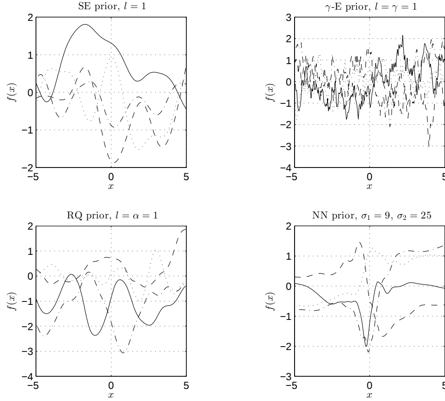
Fig. 1 Examples of functions drawn at random from Gaussian process priors using the covariance functions in Table 10. In the case of the NN prior the parameter matrix is \mathbf{S} = \text{diag}(\sigma_1, \sigma_2)
