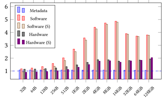
Figure 6: Allocator benchmark results on Ibex
