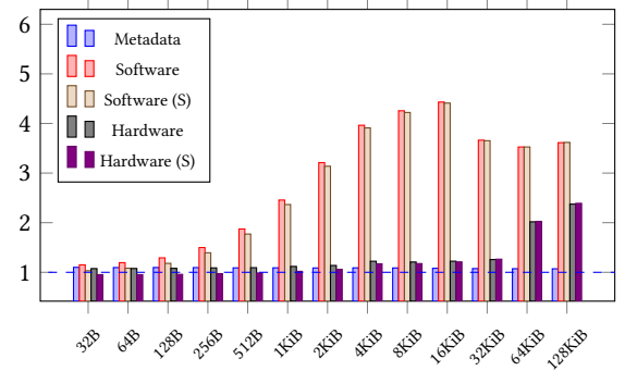
Figure 5: Allocator benchmark results on Flute
