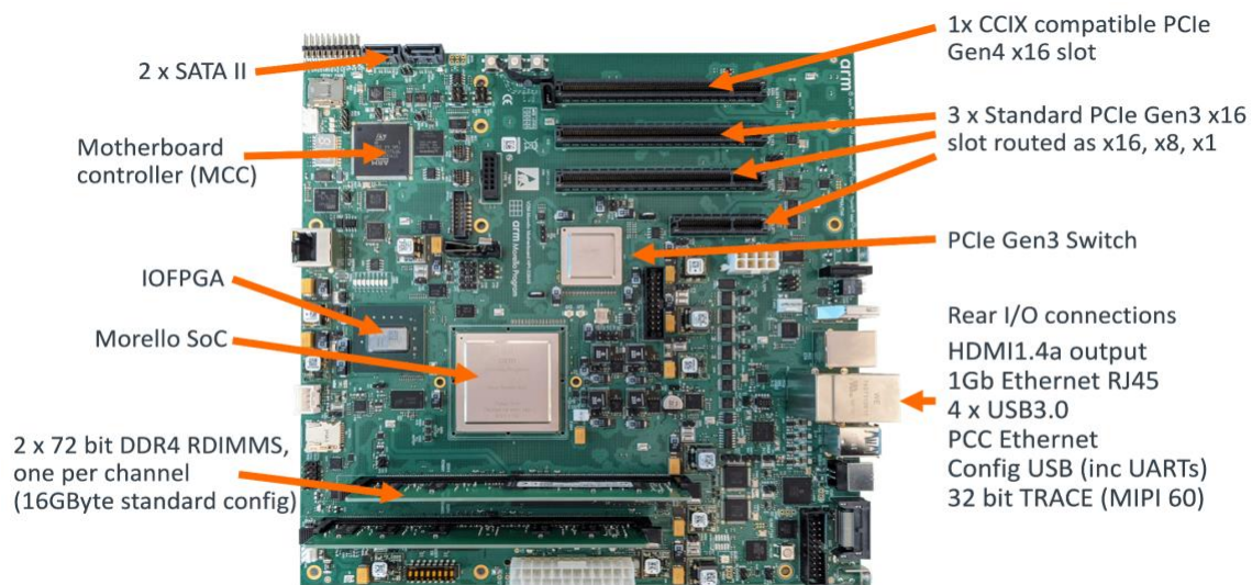
Figure 1: The features of the Morello demonstrator board
