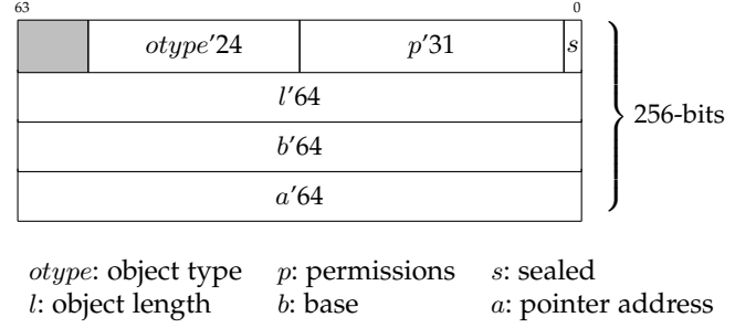
Fig. 1: CHERI-256 capability format
