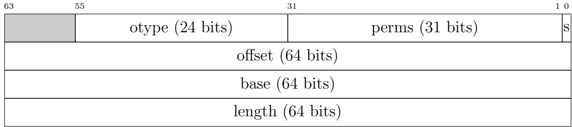
Figure 3.1: Fields of a 256-bit CHERI capability
