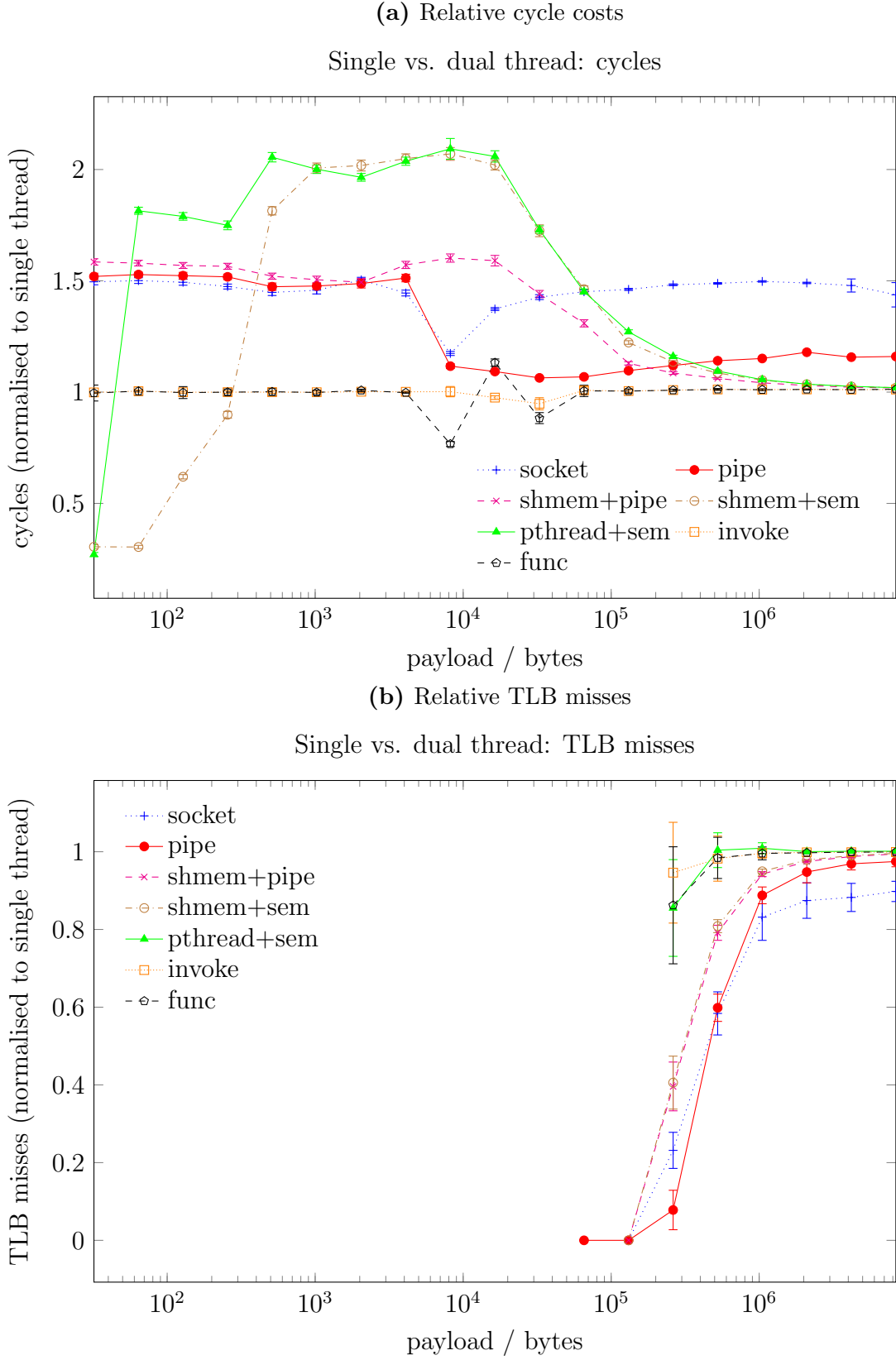
Figure 4.7: Comparison of domain crossing methods – single vs. dual thread
