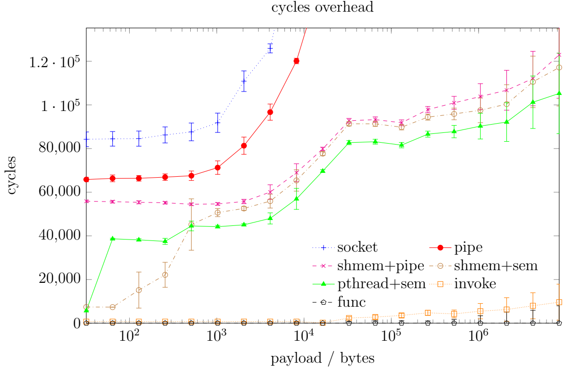
(b) Cycle overhead vs. function call (log-linear)
